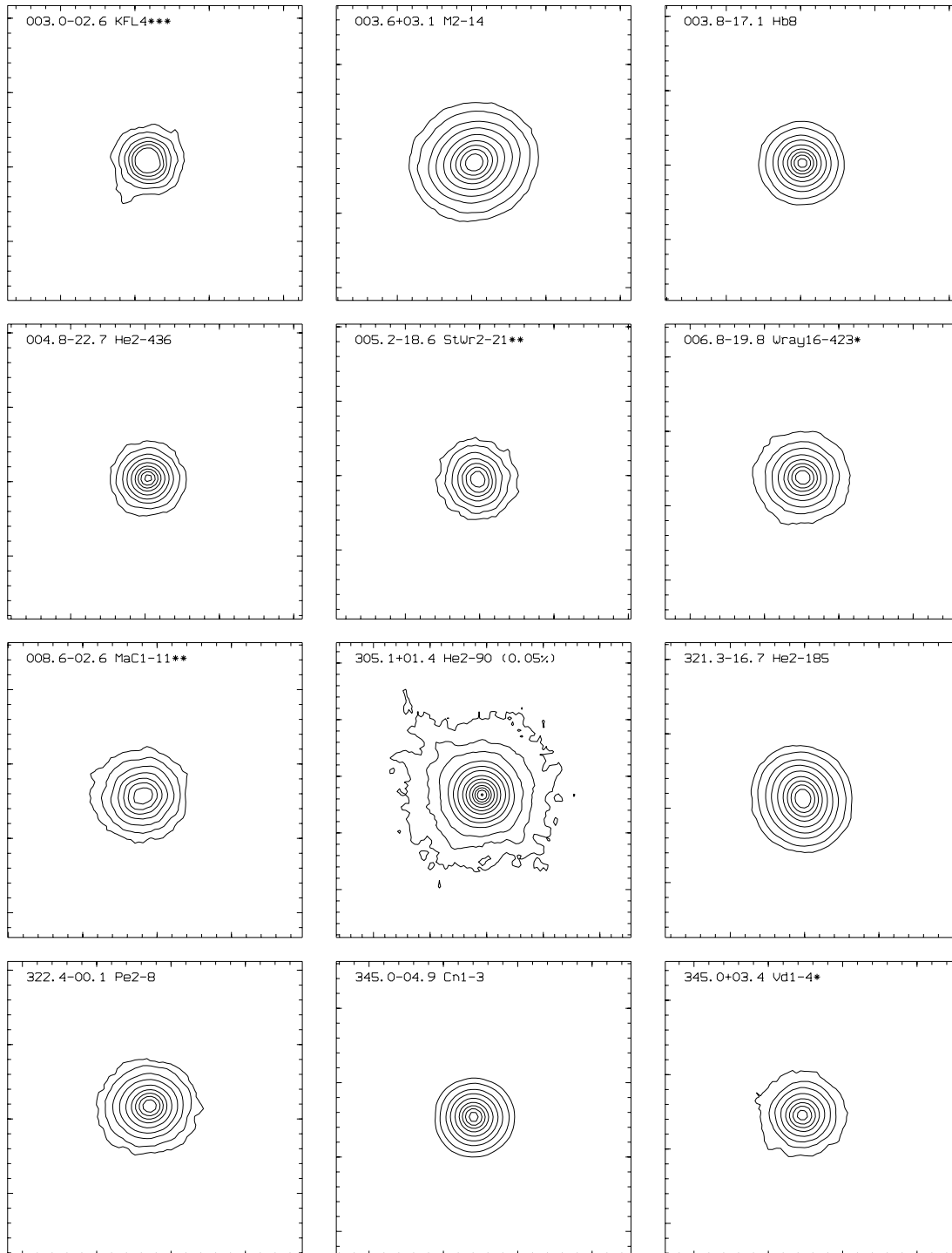
Figure A.1: Additional H\alpha image plots with contour levels at 80, 65, 50, 35, 20, 10, 5, 2, 1 per cent of the nebula peak (lowest contour level = 1, except * = 2, ** = 5, *** = 10 per cent). Actual lowest contour level plotted dependent on signal-to-noise ratio. All images are 26'' \times 26'' with north up and east to the left. To filter the noise, the images have been smoothed with a 3 pixel ( 0''.81 ) box.
