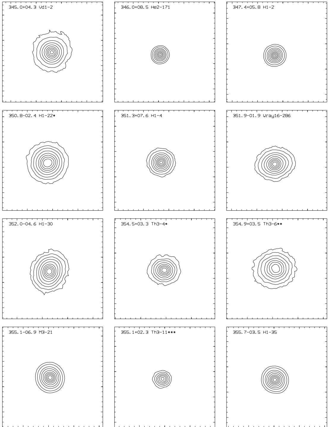
Figure A.1 (continued): Additional H \alpha image plots with contour levels.
