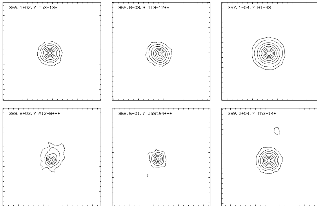
Figure A.1 (continued): Additional H \alpha image plots with contour levels.
